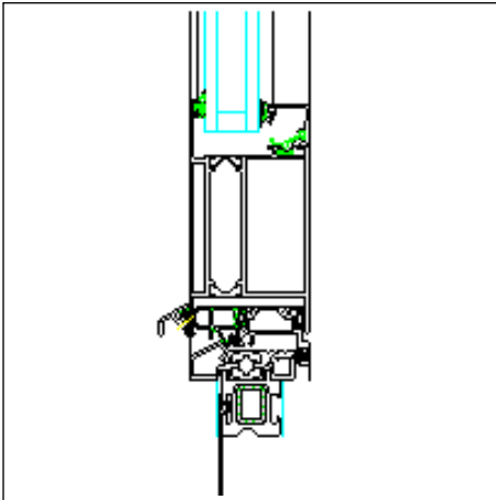
Sill attachment, inward opening Sill profile 100/125
