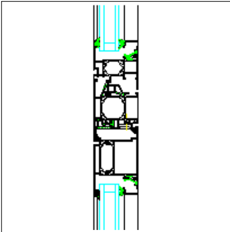
Inward opening door with toplight
