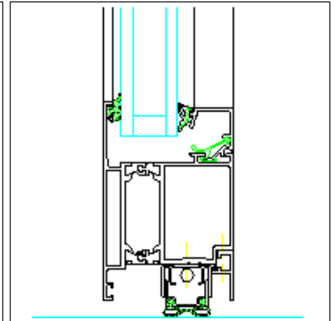
Sill attachment, outward opening with automatic door seal
