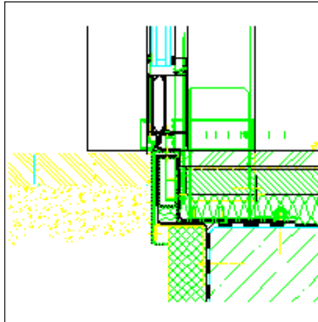
Bottom façade attachment outward opening
