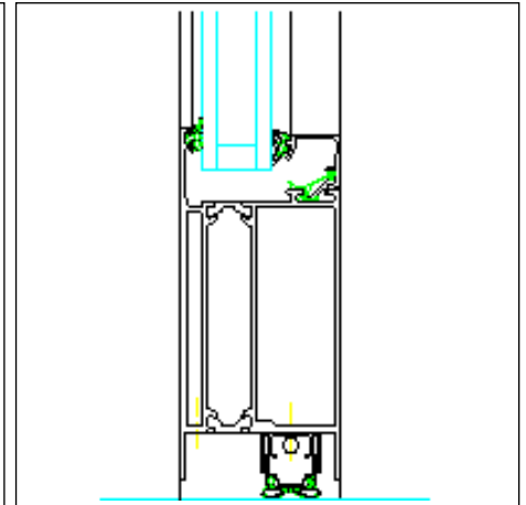
Sill attachment inward opening Automatic door seal
