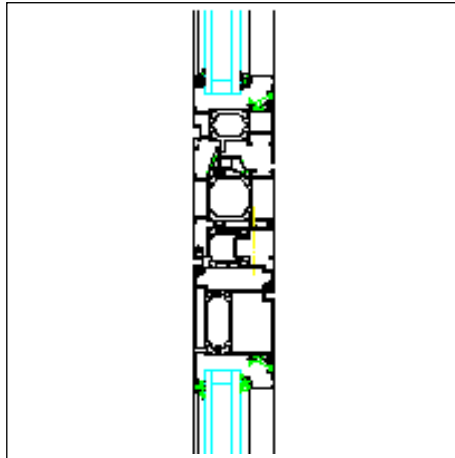
Outward opening door with toplight
