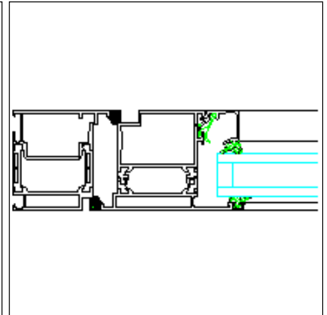
Panic door, flush-fitted door leaf
