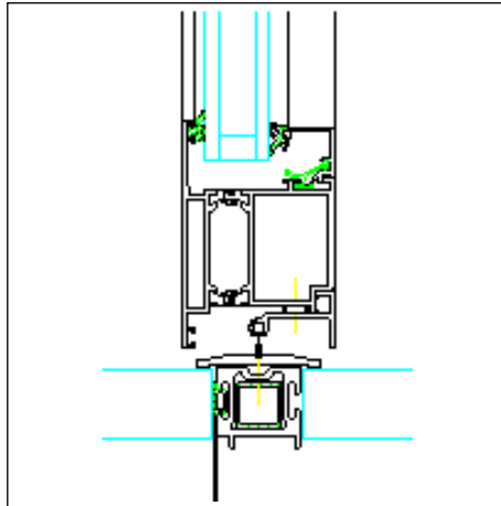
Sill attachment outward opening
