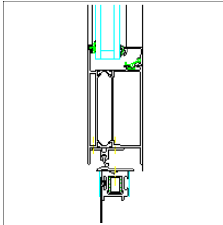
Sill attachment ,inward opening Sill profile 117/142
