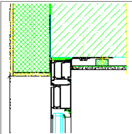
Top attachment, inward opening
