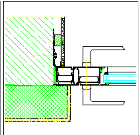
Side wall attachment, inward opening
